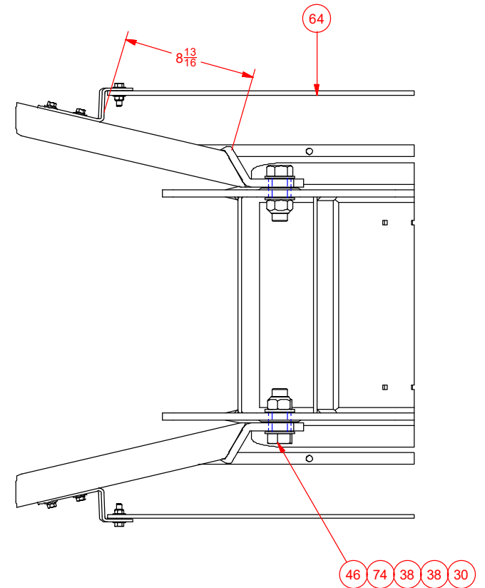
SECTION AC-AC
