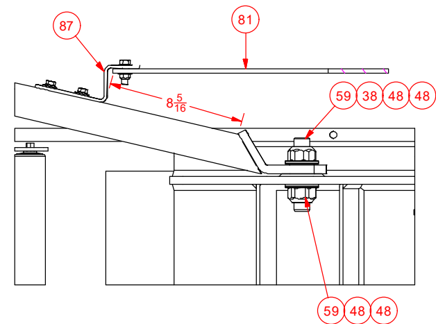
SECTION A-Y-A-Y
