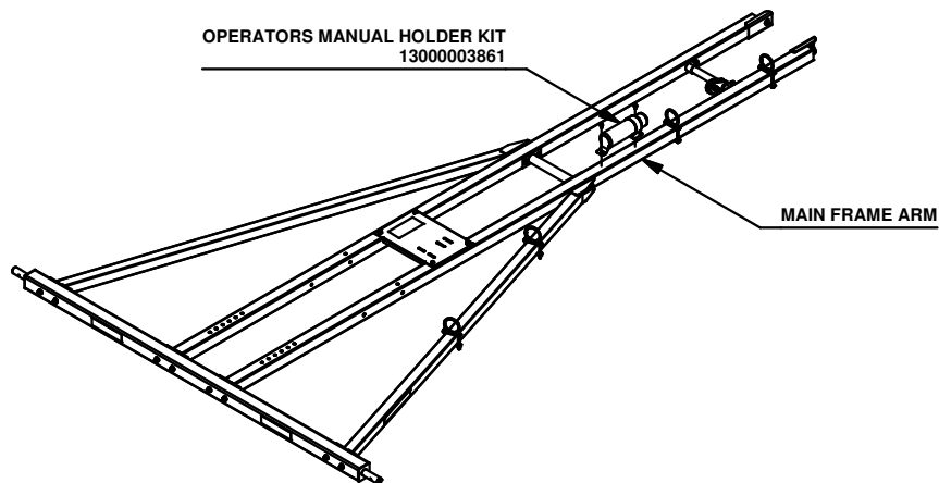
FIG 51.1 PARTS REMOVED FROM VIEW FOR CLARITY
