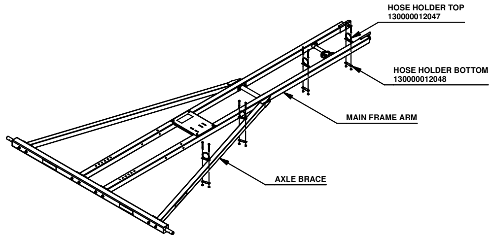
FIG 50.1 PARTS REMOVED FROM VIEW FOR CLARITY
